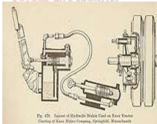
Fig. no. 2: Layout of Hydraulic Brake
